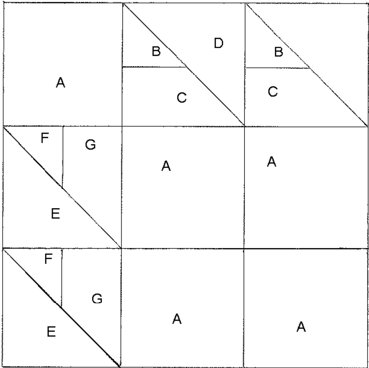
6" x 6" Block
